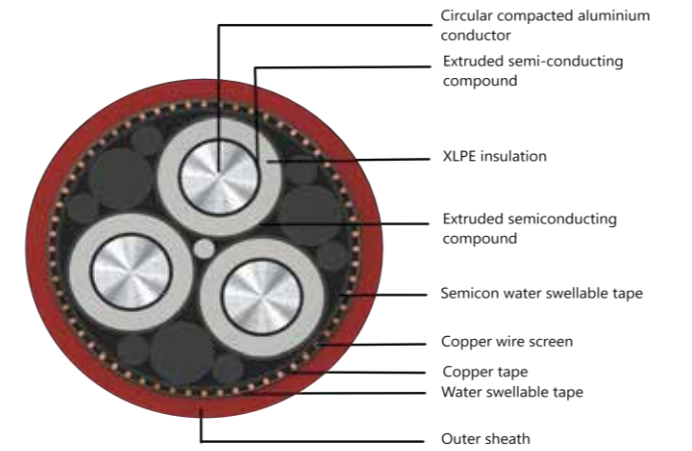
POLYCARB MV AL BS 7870-4-20 6.35/11 KV - Medium Voltage Copper wire screened Cable, 6.35/11 (12) KV AC
